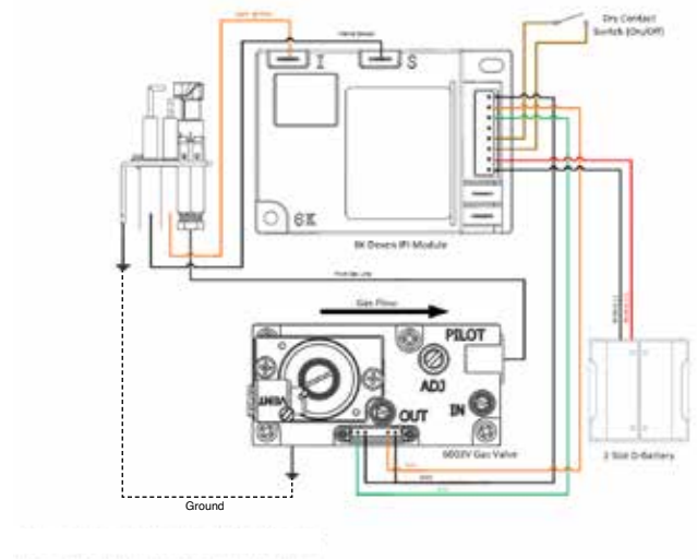
6003V - Battery Powered IPI System (6K)
