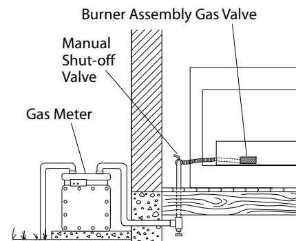
Checking Gas Joints (Natural Gas Only)
